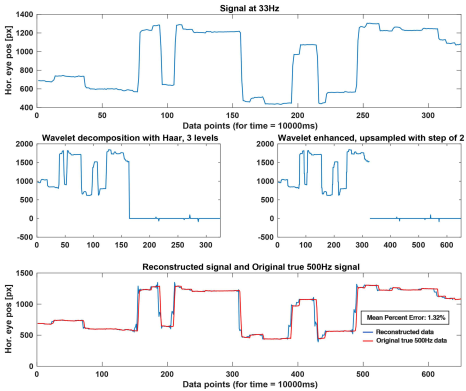
Figure 5: Results using Haar wavelet transform and nearest neighbor interpolation.
